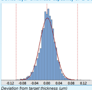
Device layer thickness capability of E-SOI® wafers
